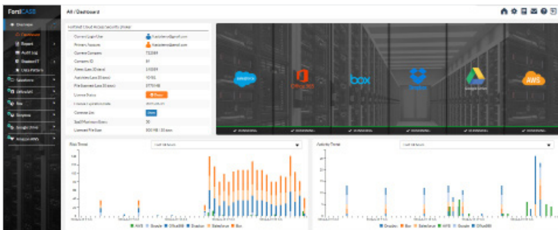
Figure 1: FortiCASB dashboard.
