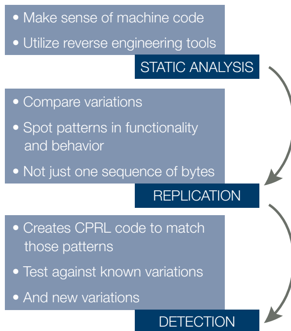
FIGURE 4 – CPRL
