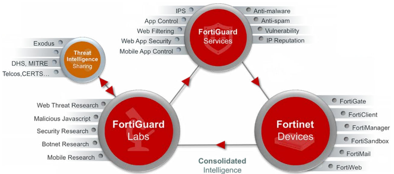
FIGURE 6 – FortiGuard
